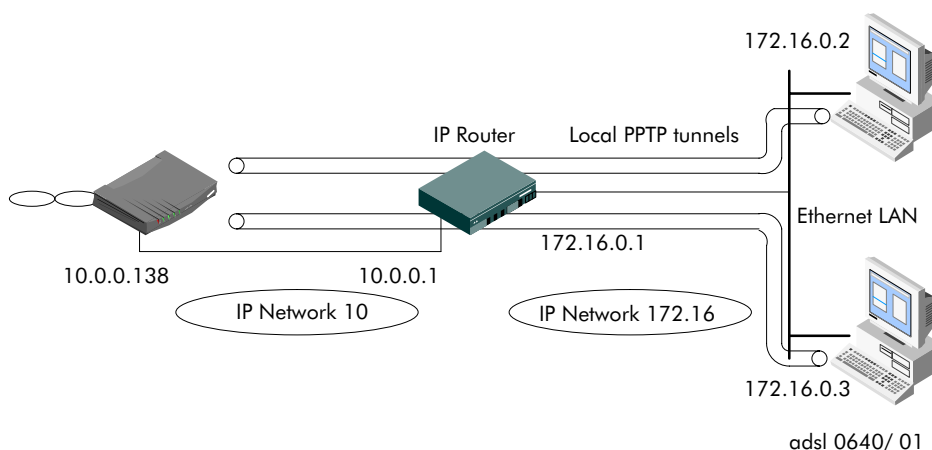
Figure 13 PPPoA-to-PPTP Advanced Network
