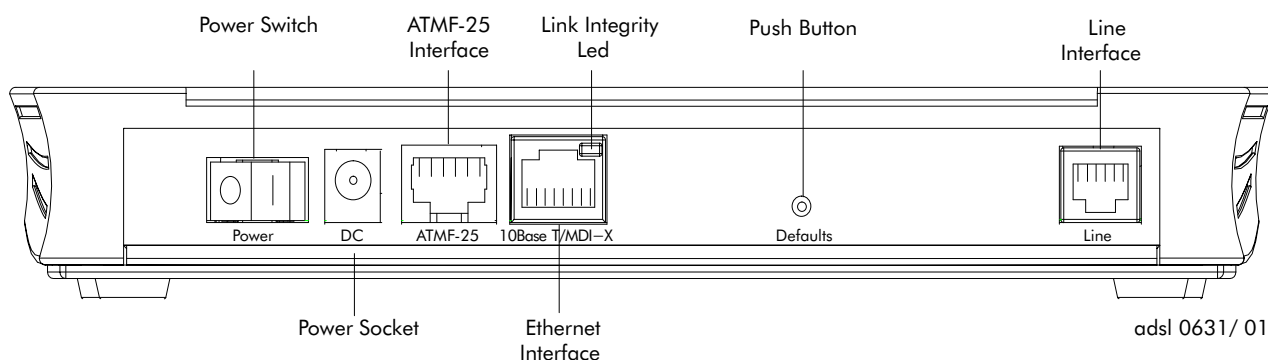
Figure 4 Rear Panel of the STHome
