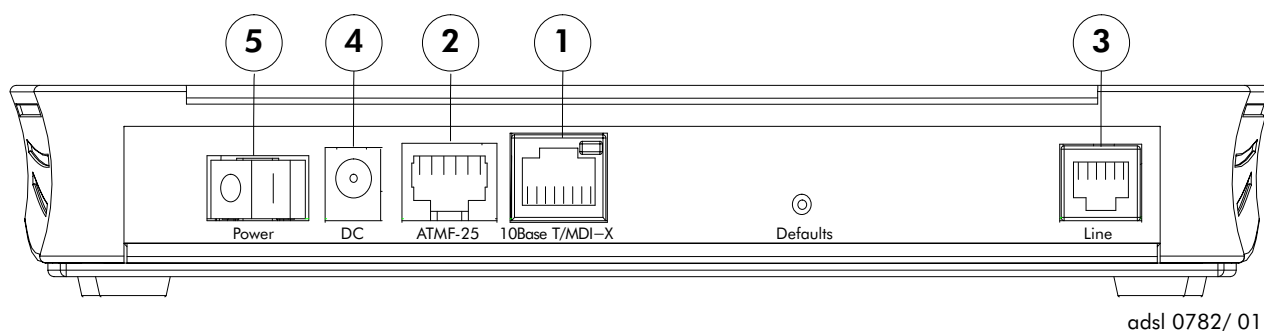
Figure 9 Rear View for connecting the STHome
